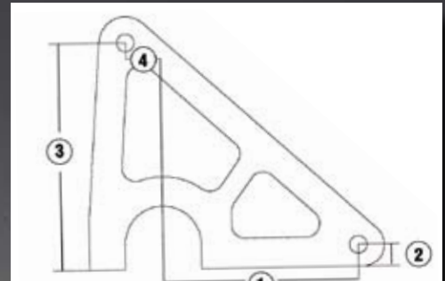
Combo Arm Dimensions
